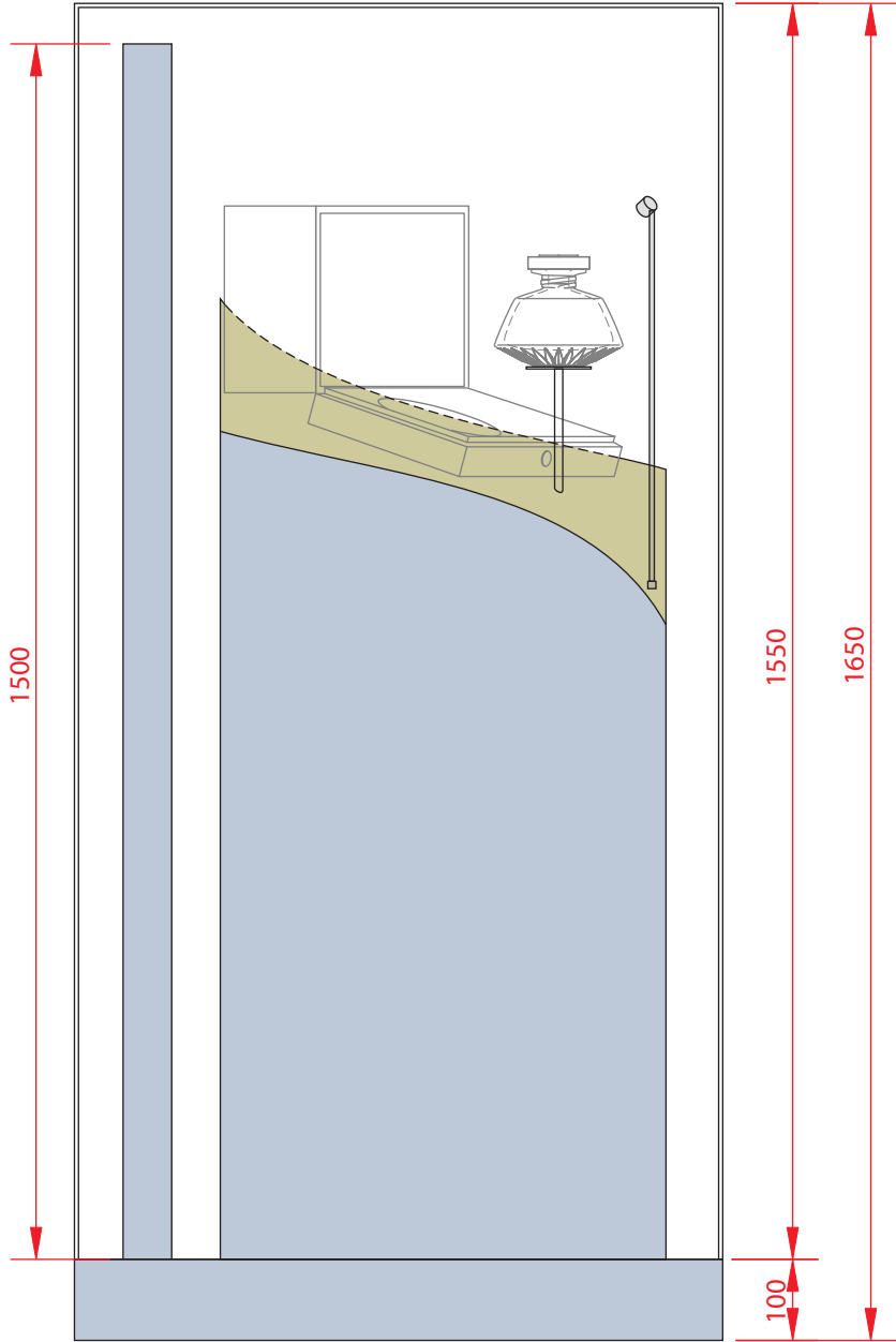
LEFT VIEW Scale 1/10 dimension mm
